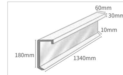
측면후레싱 10 x 180 x 60 x 30 mm
