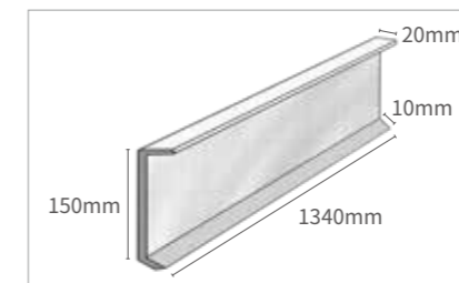
처마후레싱 20 x 150 x 10 mm
